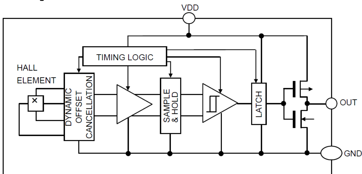
Figure 3, Block Diagram of AS1816
