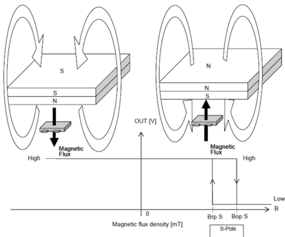
Fig 4, Magnetic Operation Characteristic of AS1816
